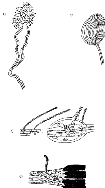
Figure 3. Schematic representation of proprioceptive mechanoreceptors: a) Ruffini ending, b) Pacinian corpuscle, c) muscle spindle receptors, and d) Golgi tendon organs. (Adapted from Willis and Grossman. 34 )
